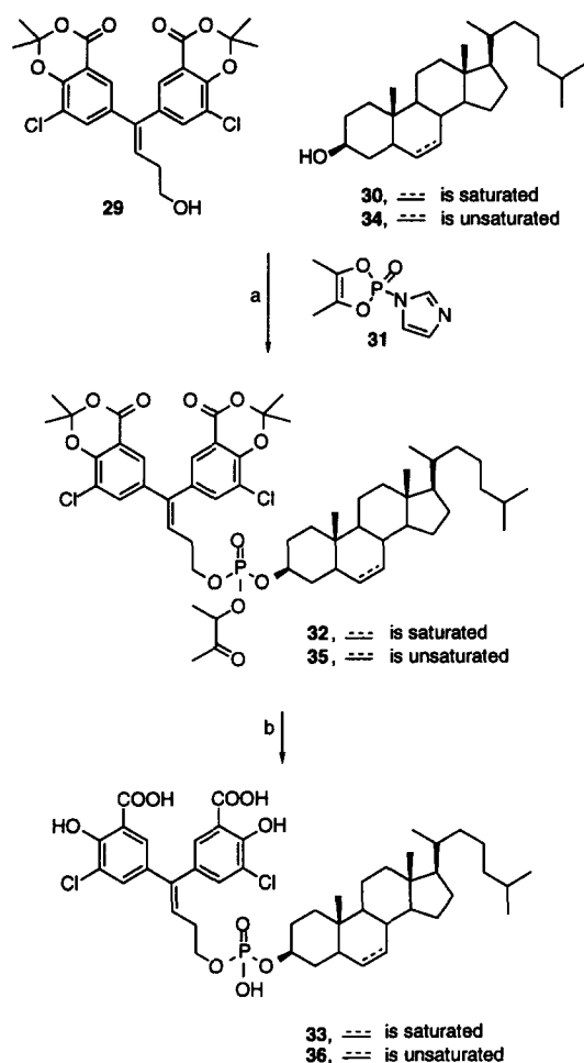
Scheme 5. Reagents and conditions: (a) \text{CHCl}_3 , -10\text{ }^\circ\text{C} (15 min), 23\text{ }^\circ\text{C} (2.5 h); (b) (1) aq. \text{K}_2\text{CO}_3 , 1,4-dioxane, reflux (3 h); (2) 3 N HCl, 23\text{ }^\circ\text{C} (1.5 h).
