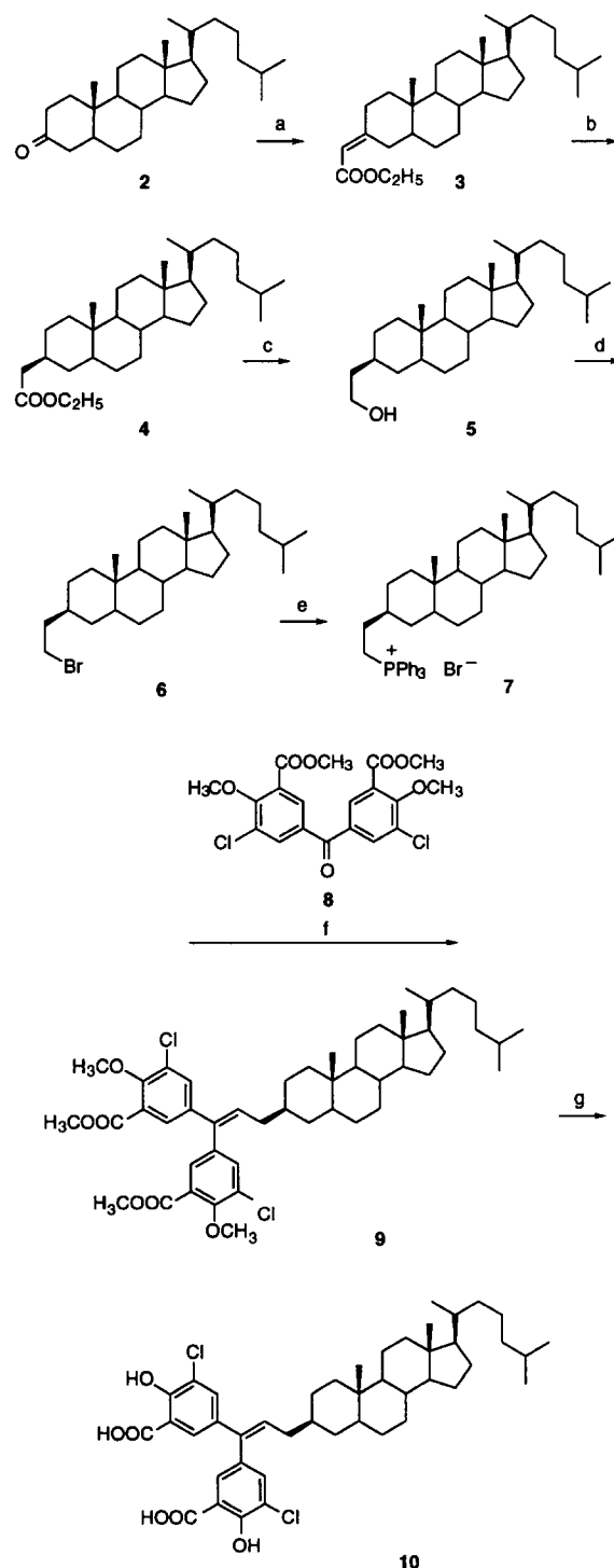
Scheme 1. Reagents and conditions: (a) (1) (\text{EtO})_2\text{POCH}_2\text{COOEt} , NaOEt, DMF, THF, 23 °C (1 h); (2) cholestanone ( 1 ), 23 °C (3 days); (b) \text{H}_2 , \text{PtO}_2 , EtOAc, 23 °C (1.5 h), 50 °C (2 h); (c) \text{LiAlH}_4 , THF, \text{Et}_2\text{O} , 0 °C (1 h); (d) \text{Ph}_3\text{P} , \text{CBr}_4 , \text{CH}_2\text{Cl}_2 , 0 °C (10 min); (e) \text{Ph}_3\text{P} , \text{PhCl} , 140 °C (24 h); (f) (1) Compound 7 , \text{NaN}(\text{SiMe}_3)_2 , THF, 0 °C (30 min); (2) compound 8 , 23 °C (2 days); (g) \text{BBr}_3 \cdot \text{Me}_2\text{S} , \text{Cl}(\text{CH}_2)_2\text{Cl} , 60 °C (24 h).
