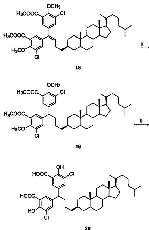
Scheme 3. Reagents and conditions: (a) \text{H}_2 , \text{PtO}_2 , EtOAc, 23^\circ\text{C} (45 min); (b) \text{BBr}_3 \cdot \text{Me}_2\text{S} , \text{Cl}(\text{CH}_2)_2\text{Cl} , 70^\circ\text{C} (8 h), 23^\circ\text{C} (12 h).
