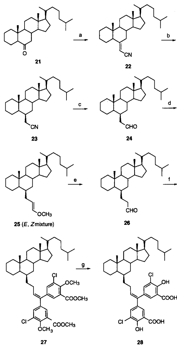
Scheme 4. Reagents and conditions: (a) (1) (EtO)_2POCH_2CN , NaNH_2 , THF, 23 °C (3 h); (2) ketone 21 , THF, 23 °C (20 h); (b) CuBr , THF, Na(CH_3OCH_2CH_2O)_2AlH_2 , PhCH_3 , 2-BuOH, 0 °C (2 h), 23 °C (5 h); (c) DIBAL, PhCH_3 , –78 °C (1.5 h); (d) (1) Ph_3P^+CH_2OCH_3 , Cl^- , NaN(SiMe_3)_2 , THF, CH_2Cl_2 , 0 °C (25 min), 23 °C (30 min); (2) 24 , THF, 0 °C (2.5 h); (e) HClO_4 , Et_2O , 23 °C (1.5 h); (f) (1) TiCl_3 –DME, Zn–Cu, DME, reflux (90 min); (2) 26 , 8, DME, reflux (1 h); (g) BBr_3 – SM_2 , ClCH_2CH_2Cl , 80 °C (3 h).
